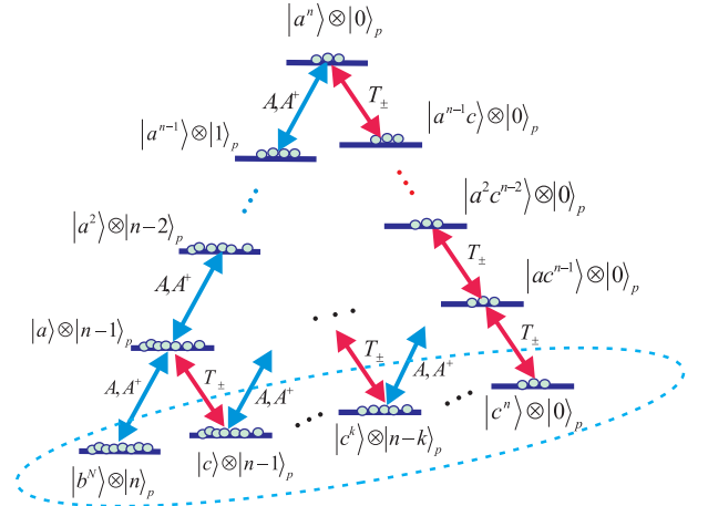
Fig. 2. The schematics of the states in the two-photon resonance system with atomic collective excitations, where |\mathbf{a}^l \mathbf{c}^m\rangle = [l!m!]^{-1/2} A^{\dagger l} C^{\dagger m} |b^N\rangle denotes there are l A -mode and m C -mode excitations in the atomic ensemble. These states in the figure are connected by the interaction of the operators A , A^\dagger , and T_\pm (also the action of the related optical fields). The dark state |d_n\rangle is a superposition of the states |b^N\rangle \otimes |n\rangle_p , |c\rangle \otimes |n-1\rangle_p , ..., |\mathbf{c}^n\rangle \otimes |0\rangle_p in the dashed envelop.
