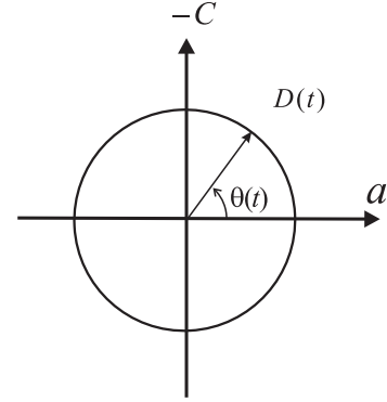
Fig. 3. Dark state polariton D = a \cos \theta - C \sin \theta is dependent on the parameter \theta(t) = \arctan g\sqrt{N}/\Omega(t) . If initially \theta(t_0) = 0 , D(t_0) = a , and the state of the total system is described as |\psi(t_0)\rangle = |b^N\rangle \otimes |n\rangle_p , then when \theta is adiabatically changed to \theta(t_1) = \pi/2 , one has D(t_1) = -C and the state is described as |\psi(t_1)\rangle = (-1)^n |\mathbf{c}^n\rangle \otimes |0\rangle_p .
