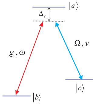
Fig. 1. The probe and control optical fields are respectively coupled to two atomic transitions with the same detuning \Delta_c . That is, such a system consisted of 3-level \Lambda -atoms ensemble and two optical fields satisfies the two-photon resonance EIT condition.
